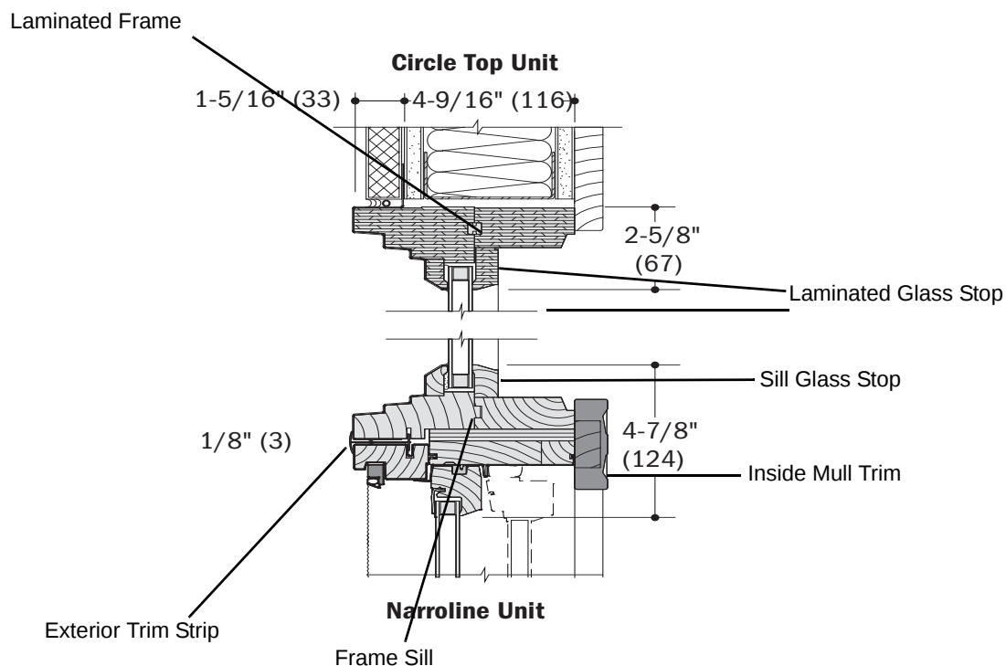
Double-Hung Circle Top™ Transom Joining
