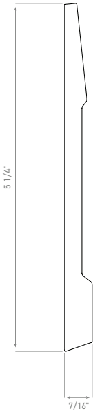
4" REVEAL BEVEL BOARD (25 boards per square)
