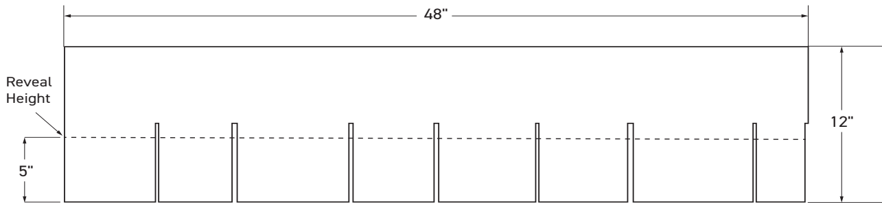
5" REVEAL STRAIGHT-EDGE SHINGLE PANEL (60 panels per square)
